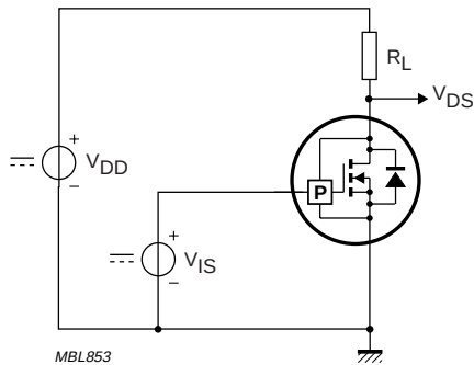
Fig 19. Test circuit for resistive load switching times.
